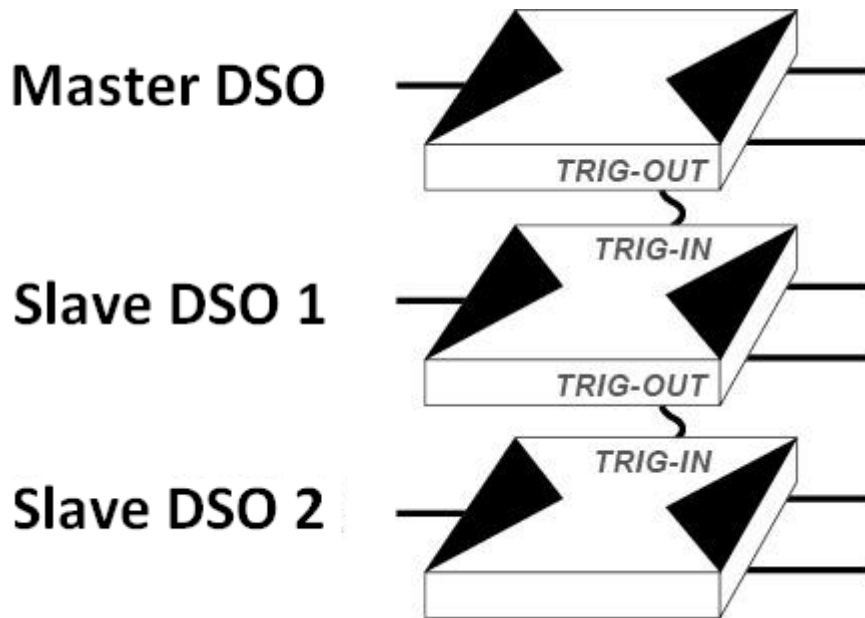
Figure: 示波器堆疊示意圖
